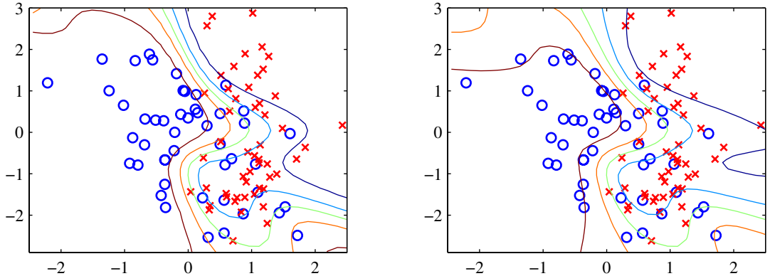
Figure 5.23 An illustration of the Laplace approximation for a Bayesian neural network having 8 hidden units with ‘tanh’ activation functions and a single logistic-sigmoid output unit. The weight parameters were found using scaled conjugate gradients, and the hyperparameter \alpha was optimized using the evidence framework. On the left is the result of using the simple approximation (5.185) based on a point estimate \mathbf{w}_{\text{MAP}} of the parameters, in which the green curve shows the y = 0.5 decision boundary, and the other contours correspond to output probabilities of y = 0.1, 0.3, 0.7 , and 0.9 . On the right is the corresponding result obtained using (5.190). Note that the effect of marginalization is to spread out the contours and to make the predictions less confident, so that at each input point \mathbf{x} , the posterior probabilities are shifted towards 0.5, while the y = 0.5 contour itself is unaffected.
