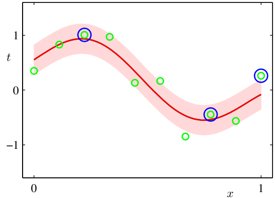
Figure 7.9 Illustration of RVM regression using the same data set, and the same Gaussian kernel functions, as used in Figure 7.8 for the \nu -SVM regression model. The mean of the predictive distribution for the RVM is shown by the red line, and the one standard-deviation predictive distribution is shown by the shaded region. Also, the data points are shown in green, and the relevance vectors are indicated by blue circles. Note that there are only 3 relevance vectors compared to 7 support vectors for the \nu -SVM in Figure 7.8.
