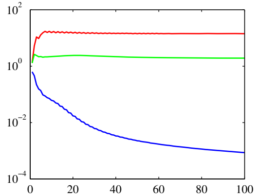
Figure 6.10 Illustration of automatic relevance determination in a Gaussian process for a synthetic problem having three inputs x_1 , x_2 , and x_3 , for which the curves show the corresponding values of the hyperparameters \eta_1 (red), \eta_2 (green), and \eta_3 (blue) as a function of the number of iterations when optimizing the marginal likelihood. Details are given in the text. Note the logarithmic scale on the vertical axis.
