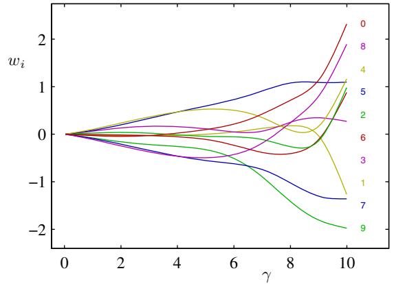
Figure 3.17 Plot of the 10 parameters w_i from the Gaussian basis function model versus the effective number of parameters \gamma , in which the hyperparameter \alpha is varied in the range 0 \leq \alpha \leq \infty causing \gamma to vary in the range 0 \leq \gamma \leq M .
