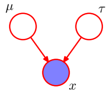
Figure 11.16 A graph involving an observed Gaussian variable x with prior distributions over its mean \mu and precision \tau .
