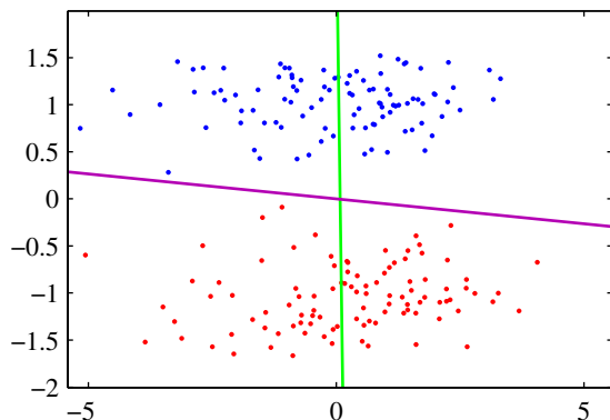
Figure 12.7 A comparison of principal component analysis with Fisher's linear discriminant for linear dimensionality reduction. Here the data in two dimensions, belonging to two classes shown in red and blue, is to be projected onto a single dimension. PCA chooses the direction of maximum variance, shown by the magenta curve, which leads to strong class overlap, whereas the Fisher linear discriminant takes account of the class labels and leads to a projection onto the green curve giving much better class separation.
