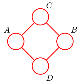
Figure 8.36 An undirected graph whose conditional independence properties cannot be expressed in terms of a directed graph over the same variables.
